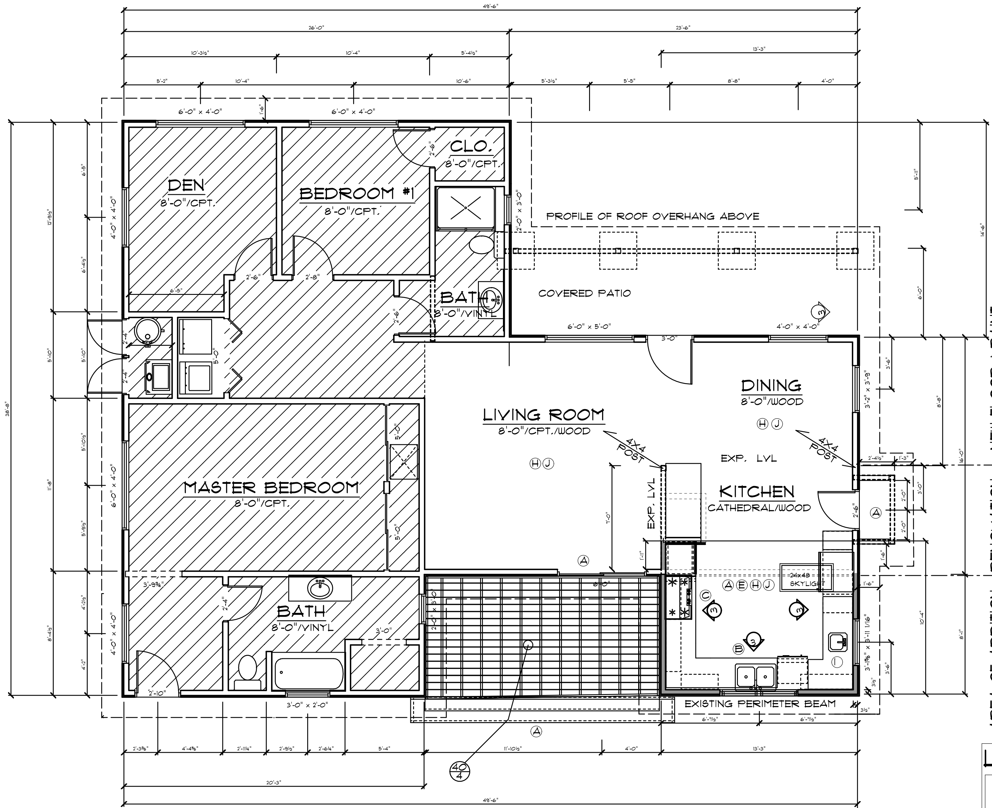
1E 1ST FLOOR PLAN - EXISTING WITH ADDITION SCALE: 1/4" = 1'-0"
